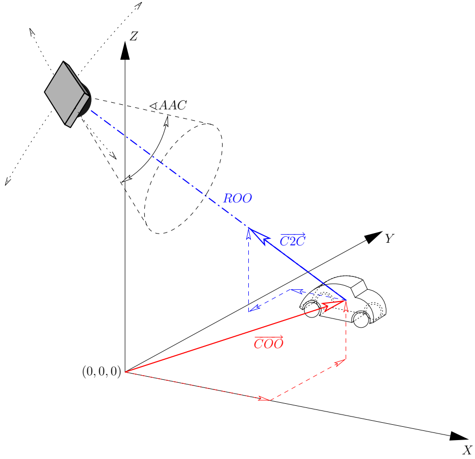
Figure 1: Camera and 3D object in the World System XYZ ; centre of orbit position vector C\vec{O}O , centre of orbit to camera direction vector C\vec{2}C , radius of orbit ROO , aperture angle of camera \angle AAC .
