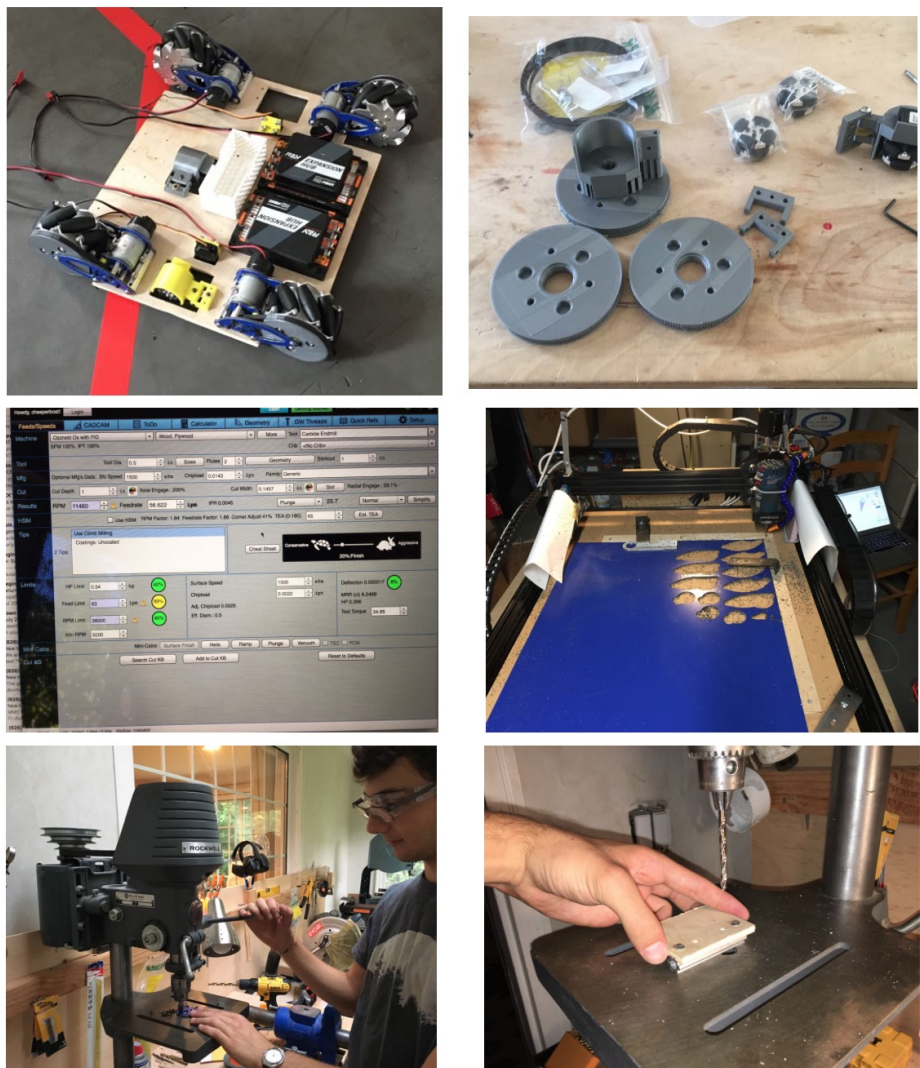
Figure 6: Building of full chassis (second iteration).
