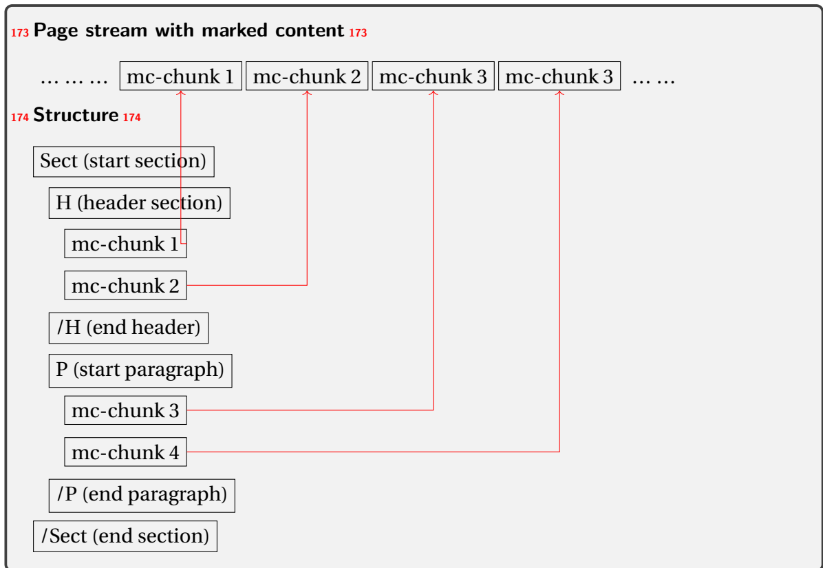
175 Figure 1: Schematical description of the relation between marked content in the page stream and the structure 175
