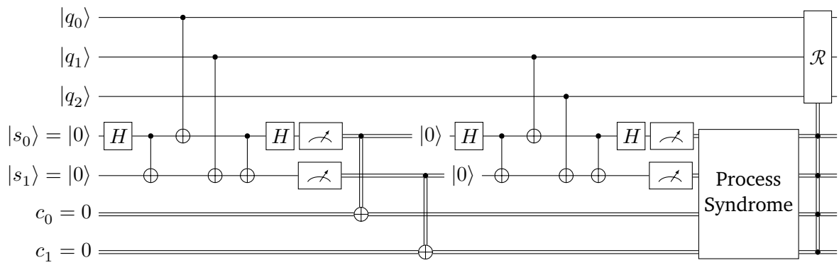
Circuit #14
